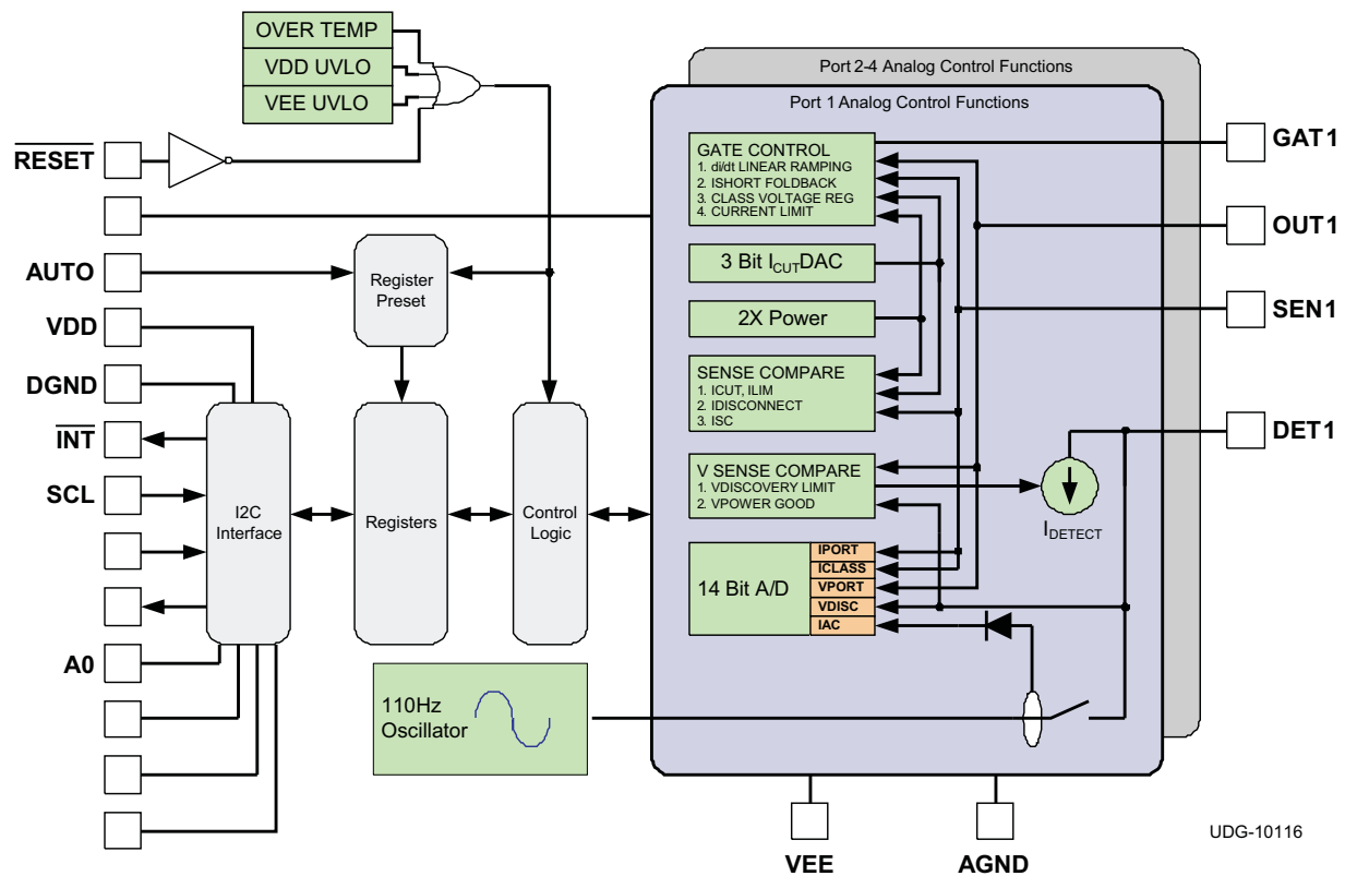
Figure 24. Block Diagram
